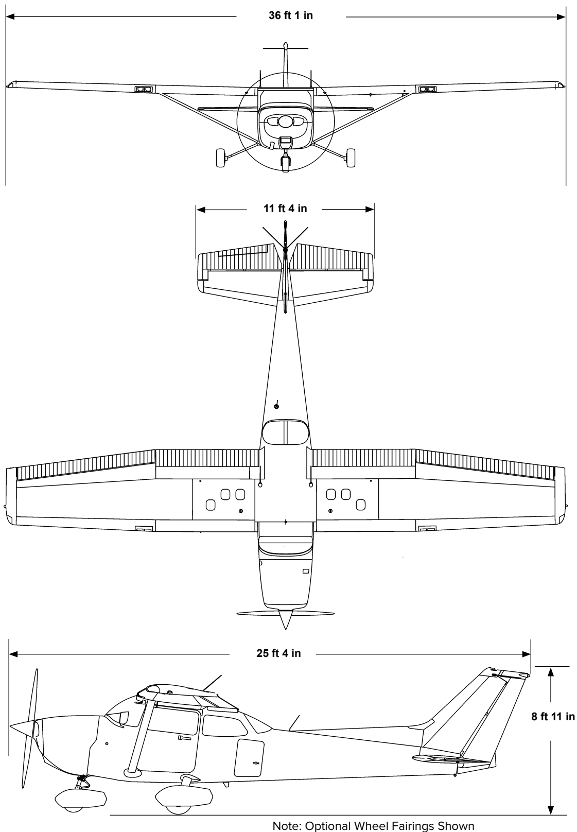
FIGURE I — CESSNA SKYHAWK EXTERIOR DIMENSIONS
